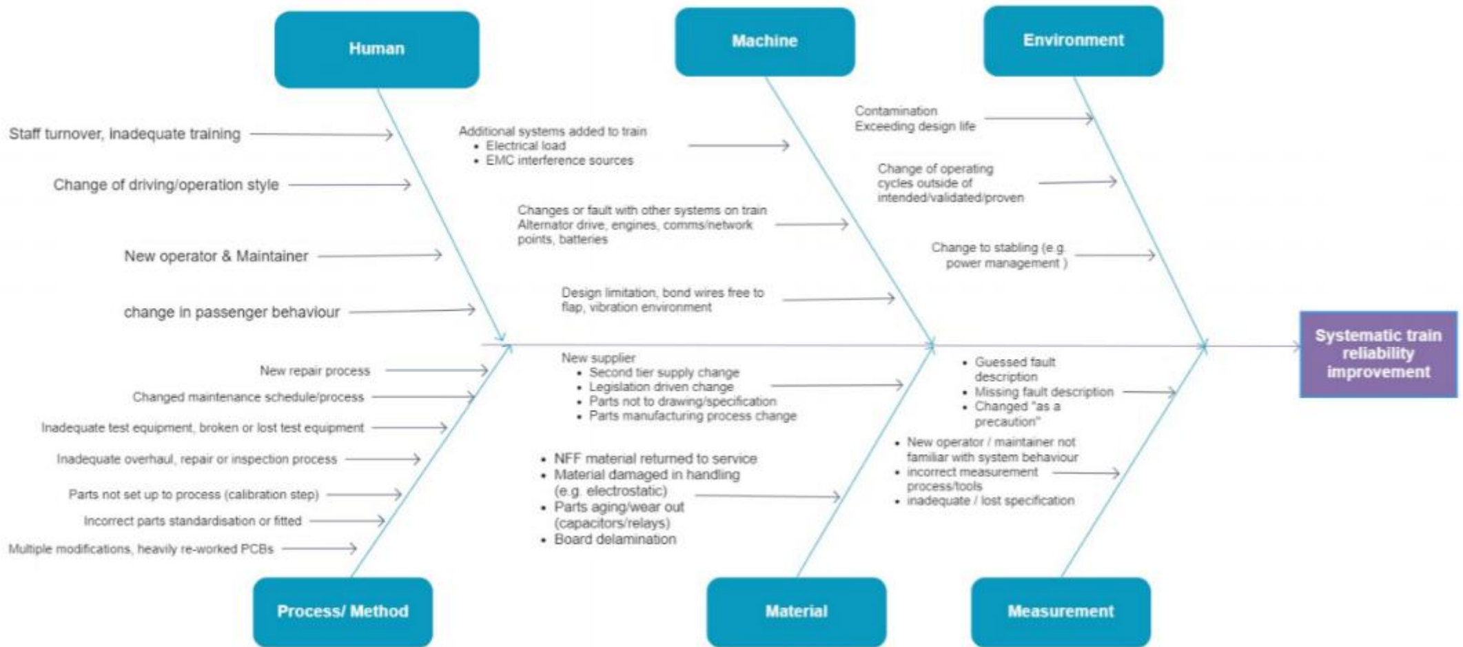
Ishikawa Diagram
